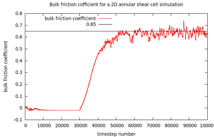
Figure 18: Time-series of the effective bulk friction coefficient from a two-dimensional annular shear cell simulation (from shearcell.py ).
