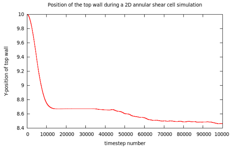
Figure 19: Time-series of the top wall position from a two-dimensional annular shear cell simulation (from shearcell.py ).
