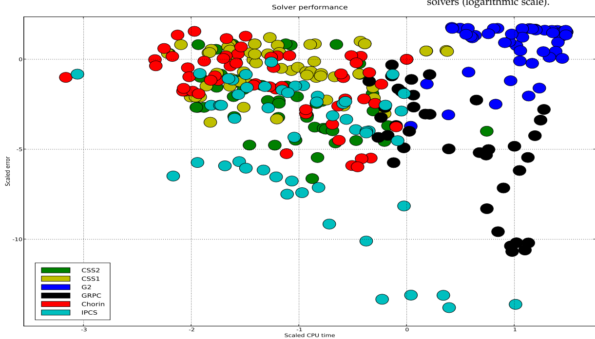
Figure 22.19: Scatter plot summarizing the results for all test problems and solvers (logarithmic scale).
