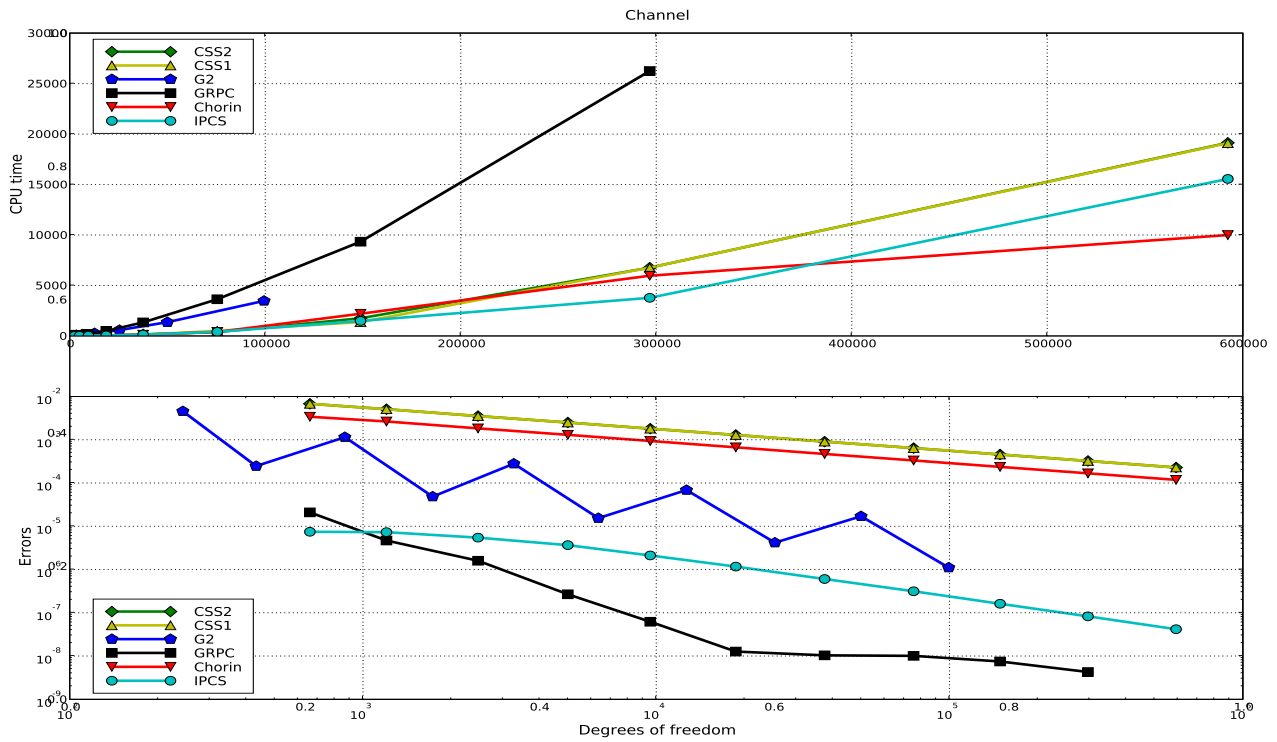
Figure 22.9: Results for the pressure-driven channel test problem.
