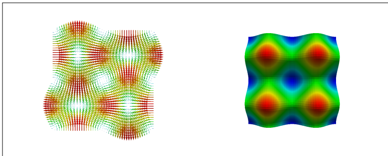
Figure 22.11: An illustration of the initial conditions for the Taylor–Green vortex test problem. On the left is the velocity field with vectors and on the right is the corresponding pressure field.
