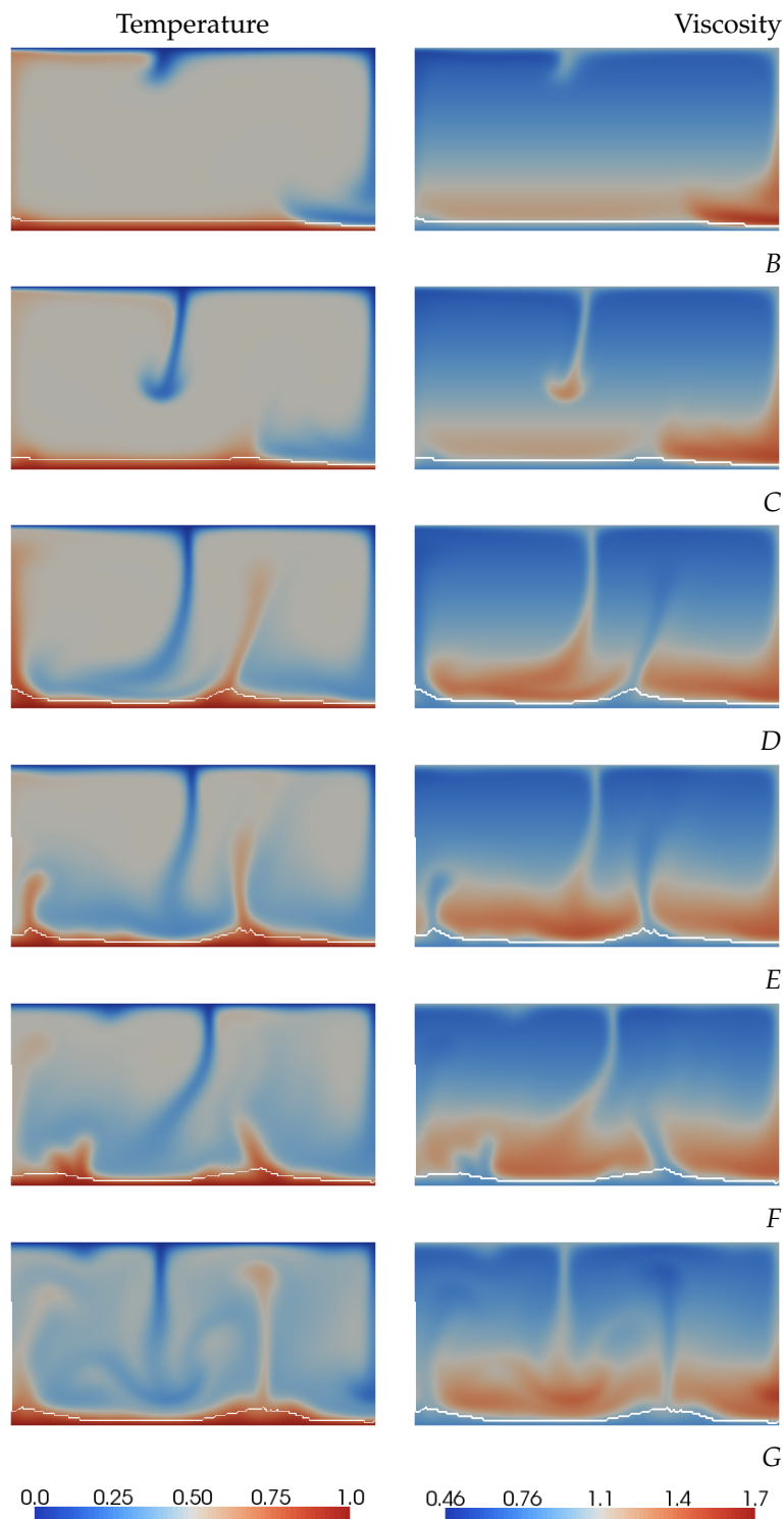
Figure 34.8: Dimensionless temperature and viscosity for turning points A to G , with composition barrier shown in white. To convert to physically relevant temperature contrast and viscosities, these values should be multiplied by dimensional \eta_0 and \Delta T from Table 34.1. The initial condition drives the system's high velocity from point A , but as the cold surface material (slab) reaches the deeper mantle, there is a retardation of the flow, towards B . The rising hot material (plume) during the stage A to B drives lateral flow of the surface causing cold material to build up until B . From B to C this cold material begins to rapidly sink, increasing u_{\text{rms}} until it is slowed by the increasing viscosity at C . However, the slab's downward motion has created a thermal instability at the base of the model, which rises between C and D increasing u_{\text{rms}} again. The pace of the material slows as the plume necks between D and E and the compositional density of the remaining material prevents it from rising further. A small plume rises from the left side of the base, increasing the u_{\text{rms}} briefly. Between E and G short-lived plumes and slabs are generated from the bottom and top boundary layers, causing small instabilities in the root-mean square velocity.
