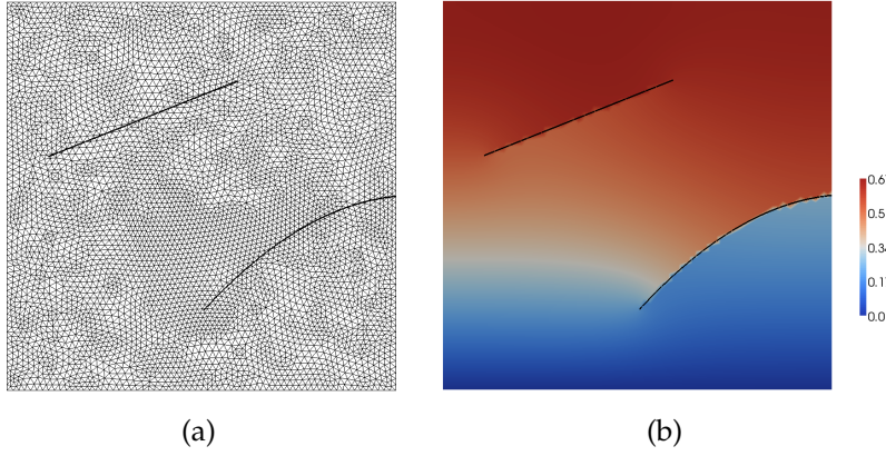
Figure 32.4: Poisson problem in two dimensions: (a) mesh and discontinuity surfaces and (b) solution contours.
