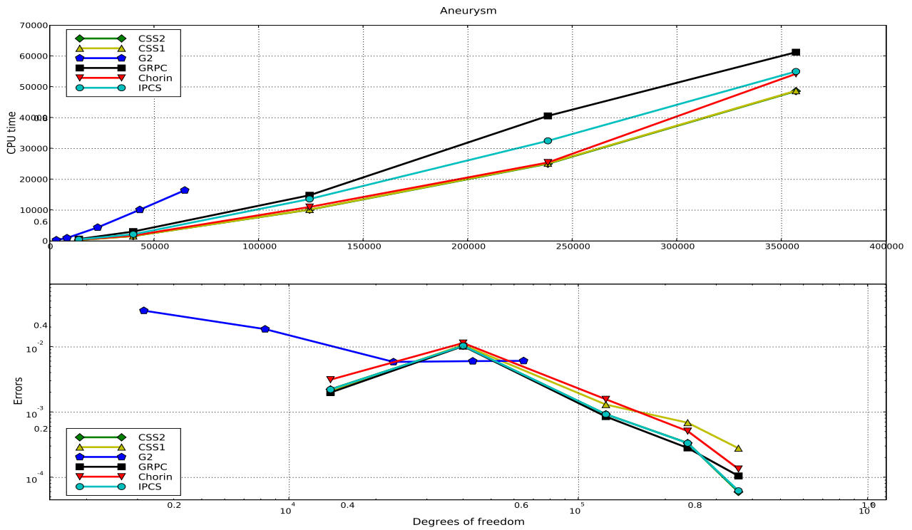
Figure 22.18: Results for the aneurysm test problem.
