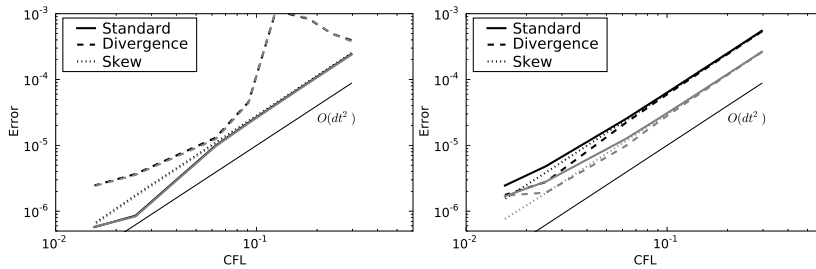
Figure 23.3: Accumulated error (23.36) vs CFL number for an integration time of 0.5 for standard, divergence and skew forms, here represented with solid, dashed and dotted lines respectively. The fully coupled and fractional step solvers are represented with gray and black lines, respectively. All results for a mesh size of N=48 . Note that in (a) the black and gray curves are practically identical (the error in the fully coupled solver is approximately 2% less throughout).
