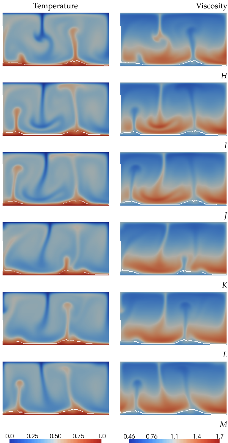
Figure 34.9: Continued from Figure 34.8, temperature and viscosity for points H to M . During the stage G-H , a second slab forms and the two downwellings merge increasing the root-mean square velocity rapidly. From H , the downwelling is impeded by the higher viscosity at depth, reducing u_{\text{rms}} until I . Then a plume arising from the bottom left rises more rapidly through the lower viscosities of the upper mantle until J . Between J and K , no new up- or downwellings occur, retarding the root-mean square velocity. From K to L a new plume increases the kinetic energy in the model, then pushes material laterally from underneath the top boundary layer until a slab begins to sink at the edge from M , increasing the velocity again.
