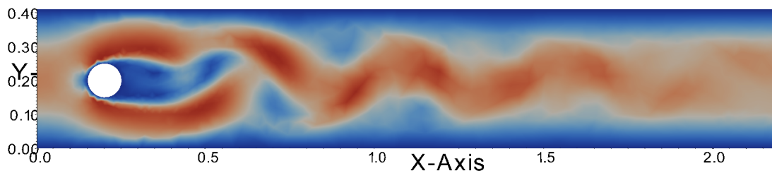
Figure 22.13: Illustration of the velocity field for the cylinder test problem at t = 5 .
