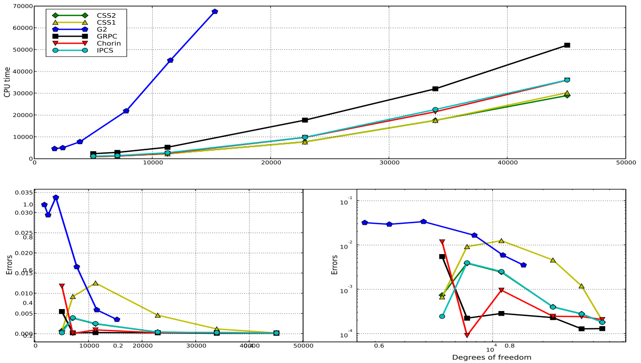
Figure 22.14: Results for the cylinder test problem.
