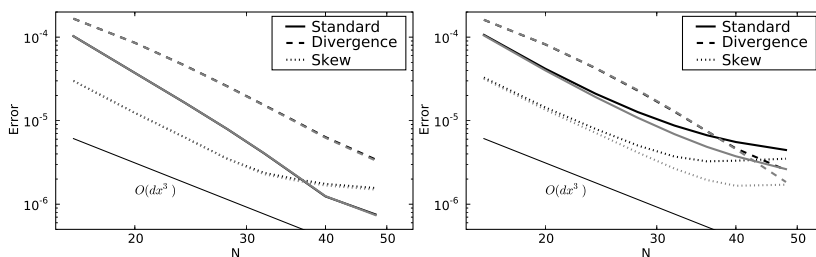
Figure 23.4: Accumulated error (23.36) vs mesh size for an integration time of 0.5. Standard, divergence and skew forms of convection are here represented with solid, dashed and dotted lines respectively. The fully coupled and fractional step solvers are represented with gray and black lines, respectively. For all results the time step used is 0.005. Note that in (a) the black and gray curves are practically identical (the error in the fully coupled solver is approximately 2% less throughout).
