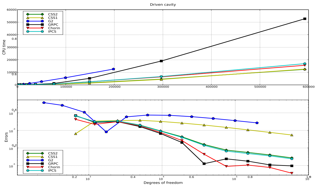
Figure 22.8: Results for the driven cavity test problem.
