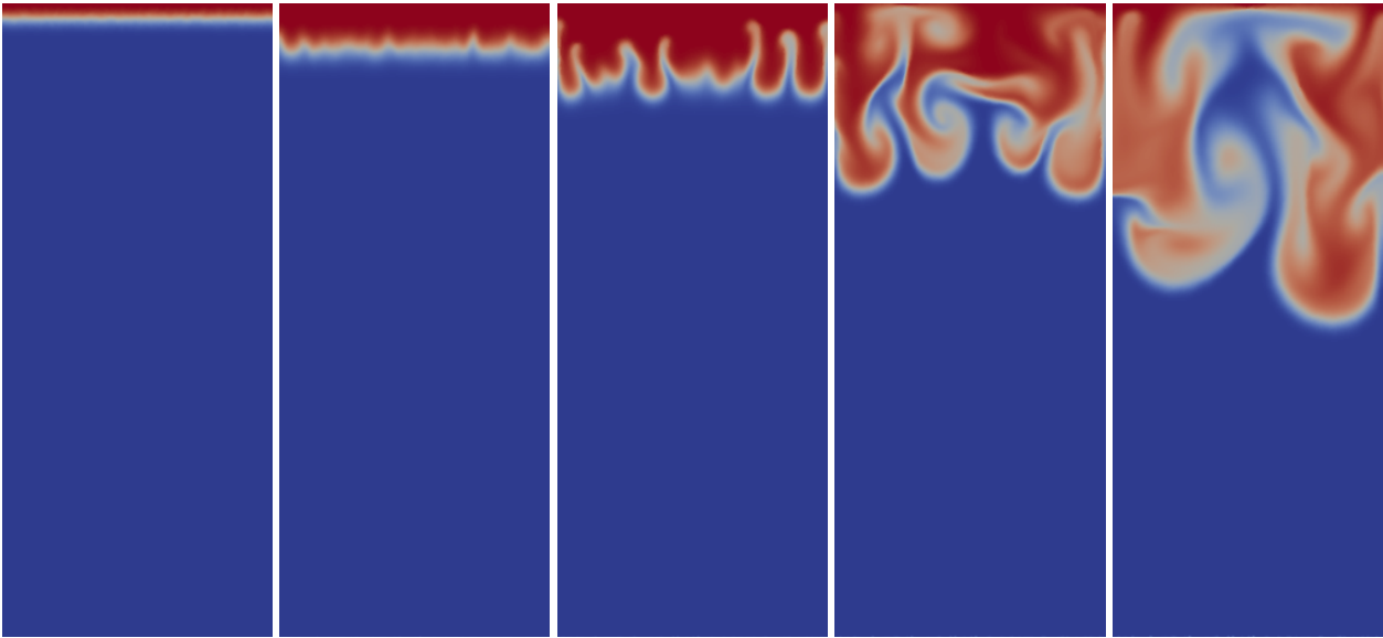
Figure 10.35: Tephra (particle) phase volume fraction at time t = 10, 30, 50, 80, 110 seconds. The onset of plumes is between 10 and 30 seconds. Note that these images are from a high-resolution version of the tephra settling example problem, with a characteristic element size of \Delta x = 0.0025 m.
